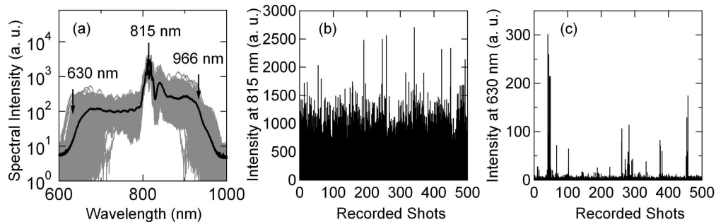
Fig. 2. (a) Typical series of 500 individual spectra (gray traces), together with the calculated mean over the same 500-shot ensemble (bold line). These results were measured at the output of a filament generated by a 15 GW ( i.e. 5 P_{cr} ) pump. (b) and (c) show time series of the intensity at (b) 815 nm in the spectrum center, and (c) 630 nm on the spectrum edge.
