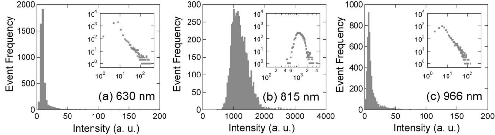
Fig. 3. Histograms at (a) 630 nm (b) 815 nm and (c) 966 nm. Insets show the same data on a log-log representation to highlight the differences in the distributions – while the distribution in (b) is bell-shaped, the distributions on the edges exhibit L-shaped characteristics.
