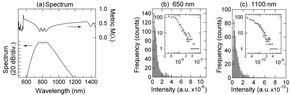
Fig. 5. (a) Mean spectrum (log scale, left axis) and Pareto metric M(\lambda) (right axis) for 1000 realizations of noise-induced SPM. Peak spectral intensity is 57 dB. (b) and (c) Histograms of spectral intensities at 650 nm and 1100 nm respectively. Insets use a log-log representation.
